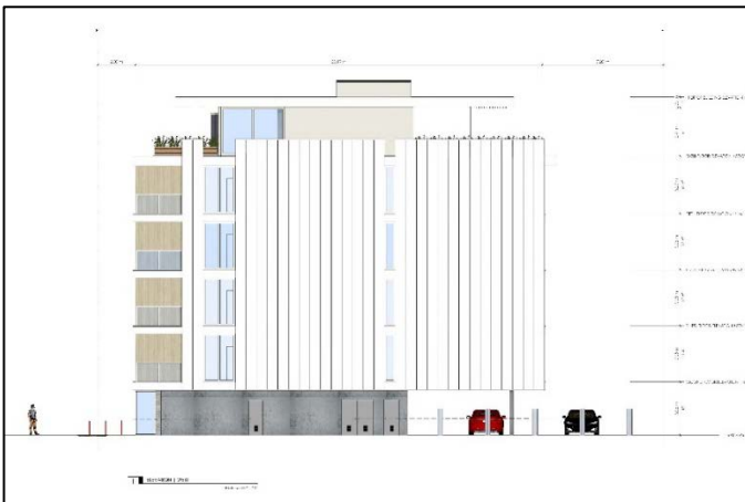
Figure 19 - West Elevation
