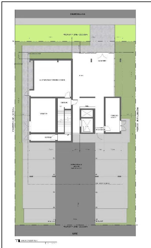
Figure 11 - Ground Level Floor Plans
