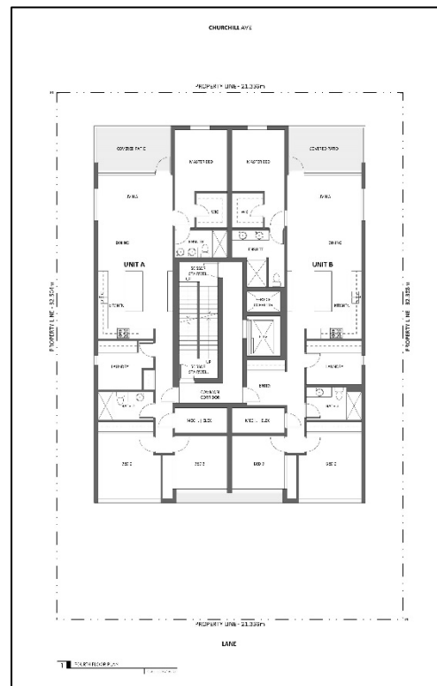
Figure 14 - Fourth Level Floor Plans
